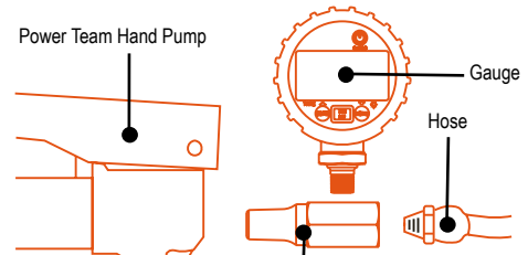
Tee adapter (No. 9670) is used for installing a gauge in line in a hydraulic circuit.
